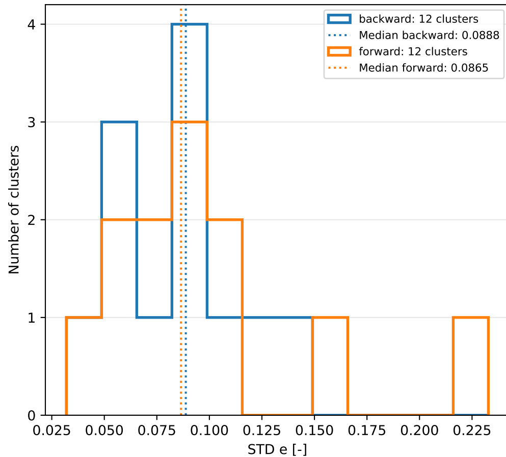
K=12 | Within-cluster STD distributions | Each cluster counts once
